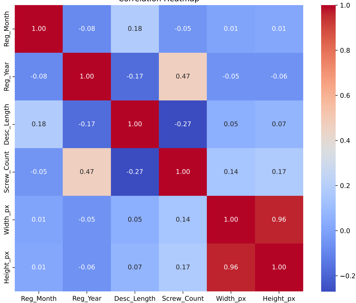
Correlation Heatmap
